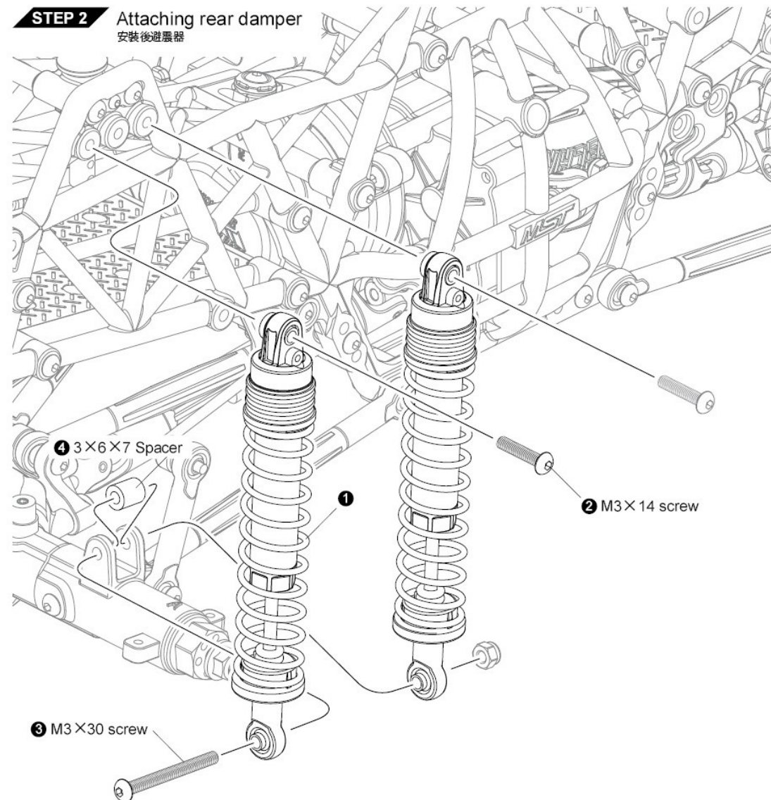
MTX damper set ×2 MTX 避震器組 230086
